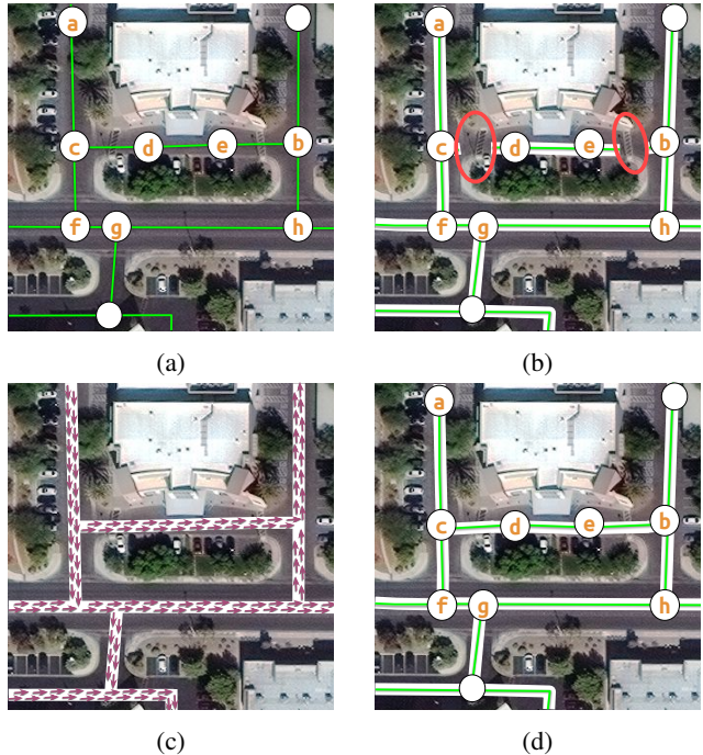
Figure 1: Road network extraction formulated as binary segmentation fails to produce topologically correct road map due to change in road appearance. (a) Annotators trace lines (highlighted nodes) along the center of roads with a traversable shortest path (a, c, d, e, b) for a \rightarrow b. (b) Fragmented road network estimated using segmentation resulting in path (a, c, f, g, h, b) for a \rightarrow b. (c) Tracing roads with orientation to achieve connectivity. (d) We extract connected and topologically correct road networks using segmentation and orientation.
